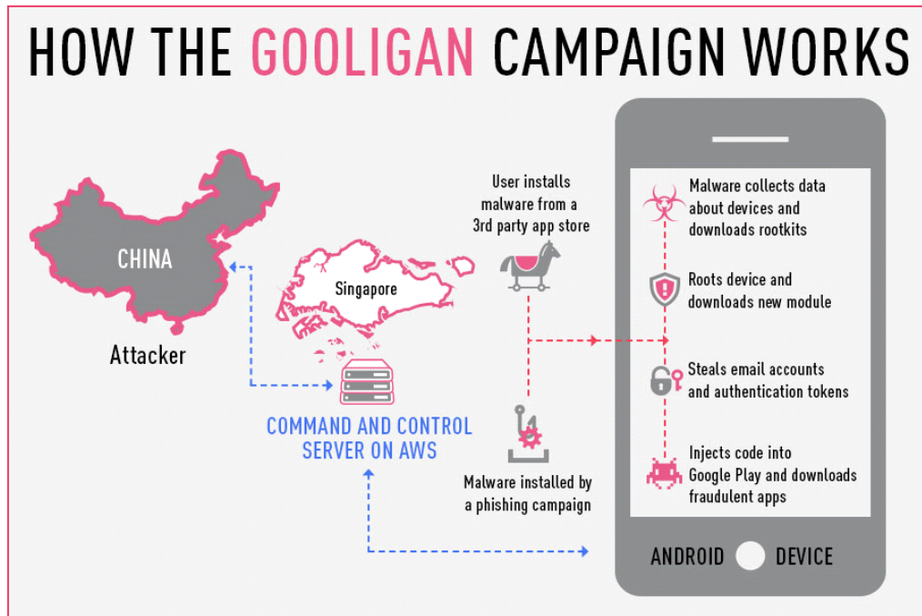
Figure 1: Malware attack flow
