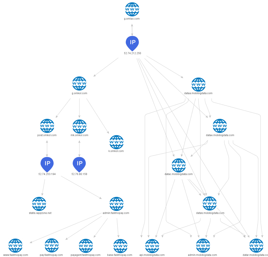
Figure 21: Network details of g.omla.com.
