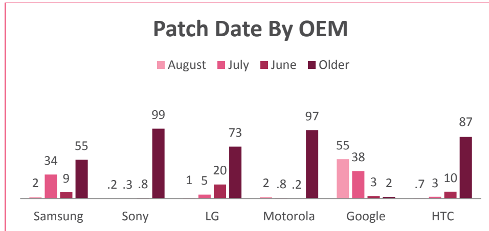
Figure 2: Android patch dates by OEMs for approximately 500,000 devices as of Aug. 10, 2016
